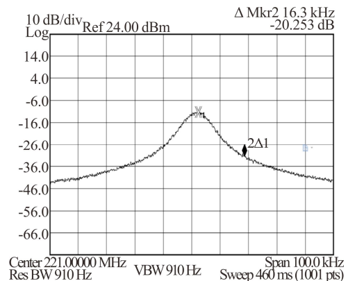
Fig.6 Spectrum of the +1 st order frequency band
