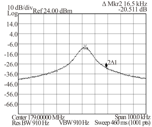
Fig.5 Spectrum of the -1 st order frequency band
