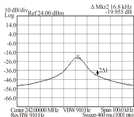
Fig.8 Spectrum of the +2nd order frequency band
