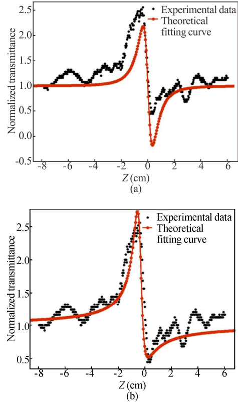
Fig.1 Closed aperture Z-scan data for DAZA polymer at the laser power of 0.6 mW using (a) SBM and (b) TLM
